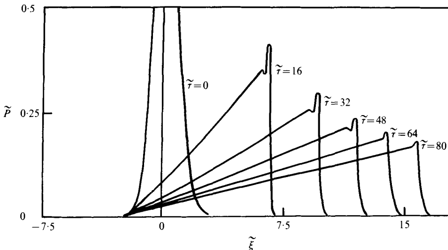
FIGURE 4. Perturbation profile for \sigma = 50 and \sigma/Re = 0.33 ; \tilde{P}(0, \xi) = \exp(-\xi^2) .
