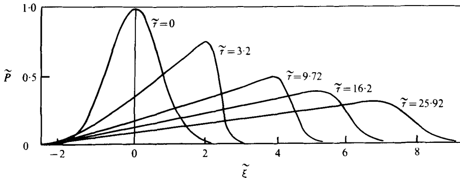
FIGURE 5. Perturbation profile for \sigma = 30 and \sigma/Re = 1.5 ; \tilde{P}(0, \xi) = \exp(-\xi^2) .
