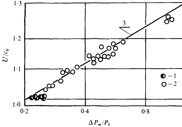
FIGURE 11. Velocity of pressure perturbation in a liquid with CO 2 bubbles. R_0 = 1.36 \times 10^{-3} m; \phi_0 = 0.99 \times 10^{-2} ; P_0 = 1.11 \times 10^5 N/m 2 ; c_0 = 109 m/s. (1) Wave packet. (2) Soliton. (3) Calculation from (12) at \gamma = 1.22 .
