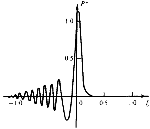
FIGURE 2. Perturbation profile for \sigma < \sigma_c and Re^{-1} = 0 .
