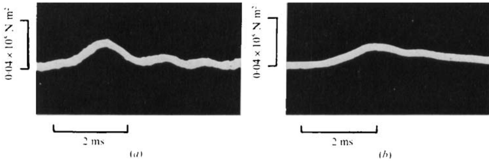
FIGURE 15. Evolution of perturbation at \sigma < \sigma_0 in a liquid with He bubbles. \sigma = 2.2 ; \sigma/Re = 0.46 ; \Delta P_0 = 0.148 \times 10^5 \text{ N/m}^2 ; l_0 = 0.033 \text{ m} .
