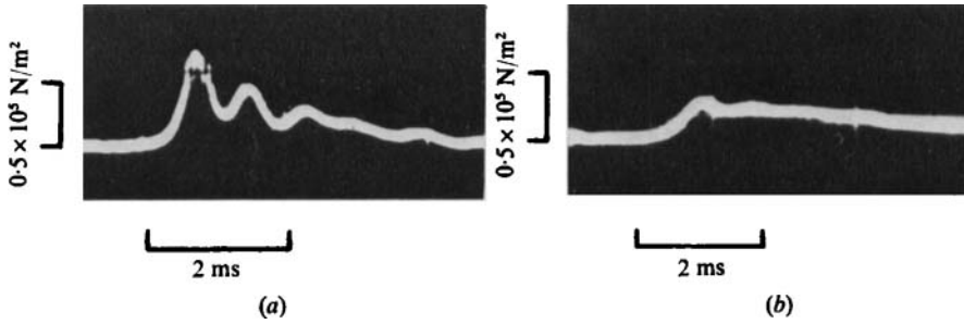
FIGURE 13. Evolution of the multi-soliton perturbation in a liquid with He bubbles. \sigma = 36 ; \sigma/Re = 0.14 ; \Delta P_0 = 1.74 \times 10^5 \text{ N/m}^2 ; l_0 = 0.15 \text{ m} .
