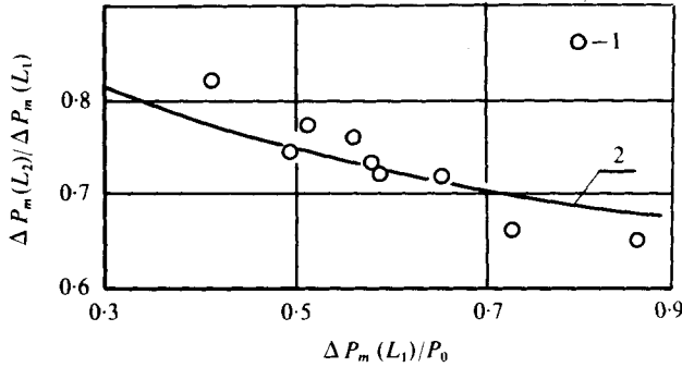
FIGURE 17. Damping of the soliton amplitude with length. Gas CO 2 , L 1 = 0.6 m, L 2 = 1.4 m. (1) Experiment. (2) Calculation from (15) for α = 6 s -1 , η = 3.3 × 10 -2 m 2 /s, γ = 1.3, β = 0.34 × 10 -2 m 3 /s.
