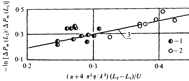
FIGURE 18. Damping of the wave packet along the test section. Gas CO 2 ; σ ≪ σ c . Experiment: (1) L 1 = 0.6 m, L 2 = 1.4 m; (2) L 1 = 0.63 m, L 2 = 1.78 m. (3) Calculation from (16) for η = 2.9 × 10 -2 m 2 /s, α = 6 s -1 , γ = 1.3.
